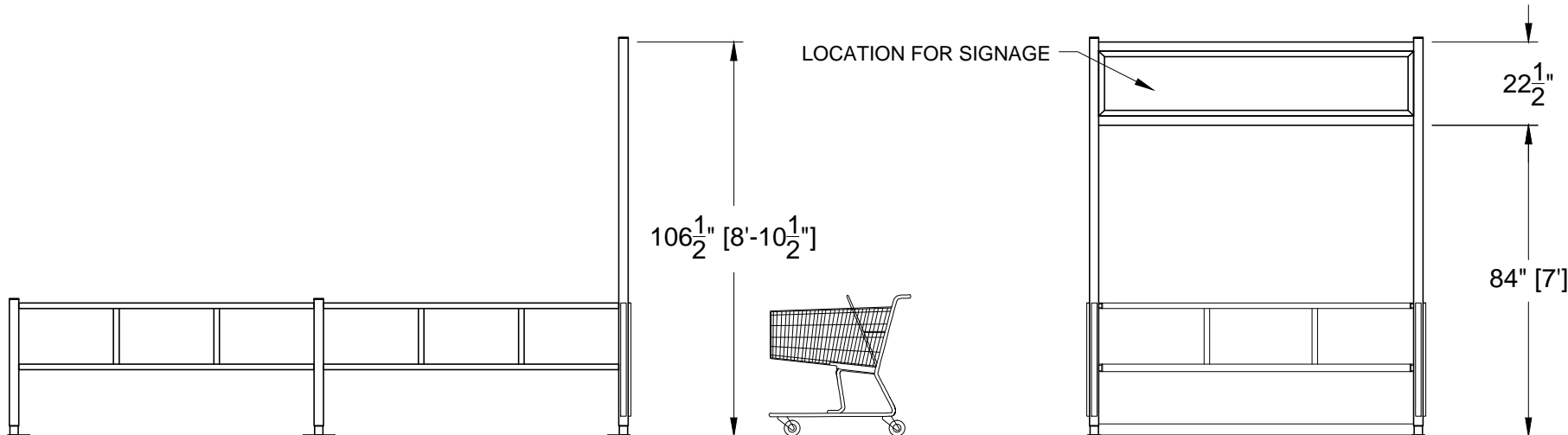
SIDE ELEVATION
